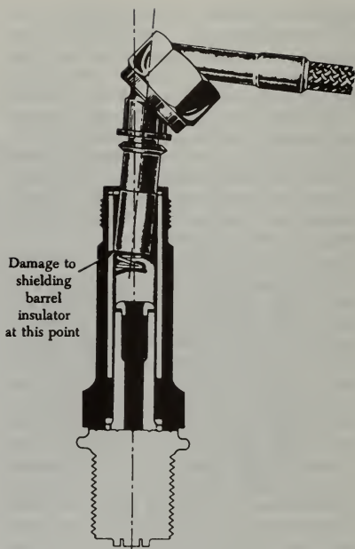
FIGURE 4-56. Improper lead removal technique.
